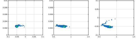
Fig. 3. Point clouds for two dimensional marginals pdfs for the three unknown parameters: \iota , m_e and v_e . From left to right: (m_e, v_e) , (\iota, v_e) , and (\iota, m_e) . The samples are given in blue and the true values is given in green. See also Fig. 2 for one dimensional plots and Tab. I for quantitative assessment.
