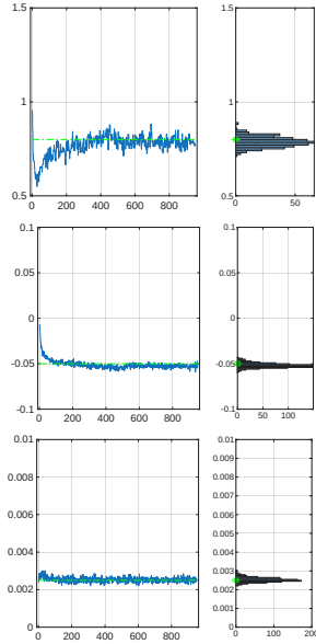
Fig. 2. Samples provided by the Gibbs algorithm as a function of iteration index (left) and as histograms (right) for the three unknown parameters from top to bottom: \iota , m_e and v_e . They are samples of one dimensional marginal pdfs. The green lines/dots give the true value. See Fig. 3 for two dimensional joint-marginal posterior and Tab. I for quantitative results.
